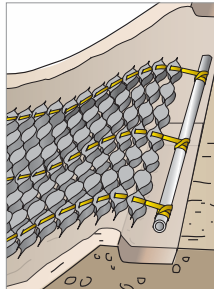
"Deadman" Pipe
