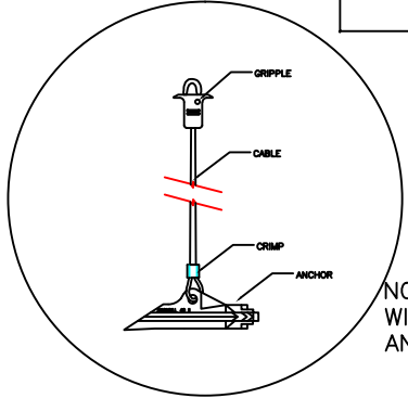
ANCHOR DETAIL
