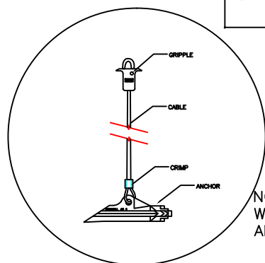
ANCHOR DETAIL
