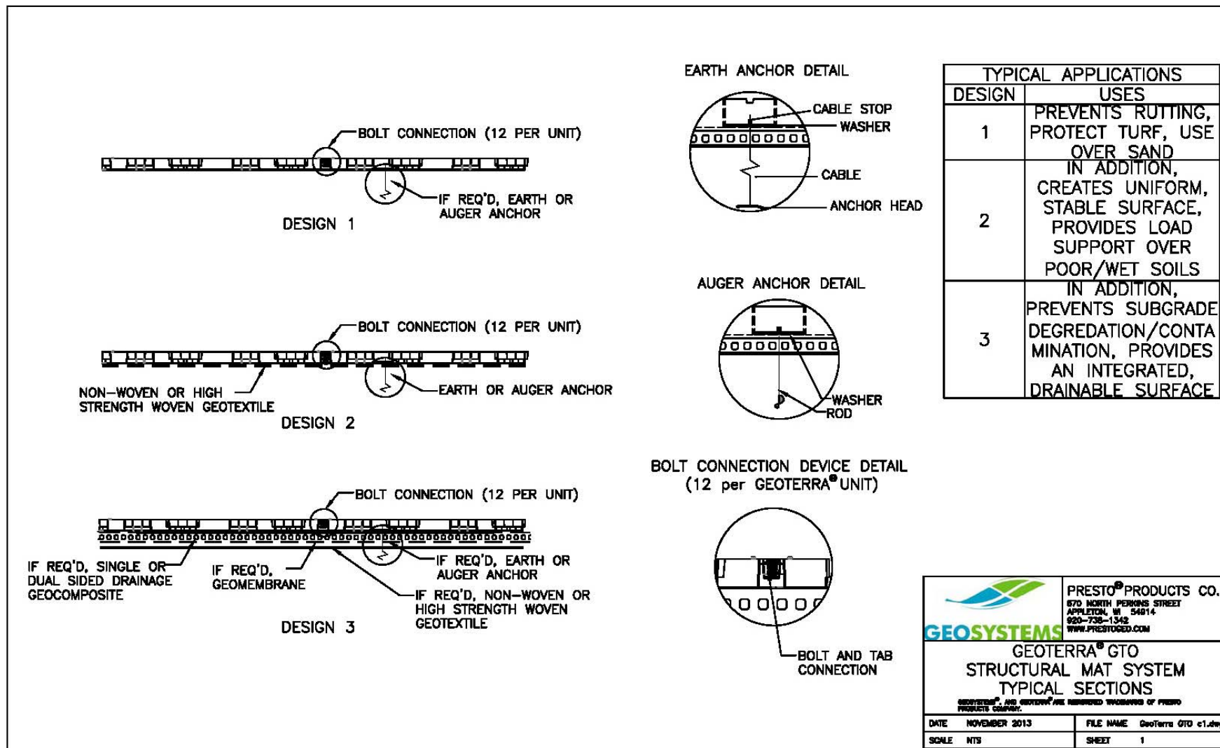
Drawing 3: GEOTERRA® GTO Design Guidelines
