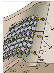
Earth anchors
