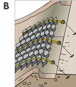
Earth anchors
