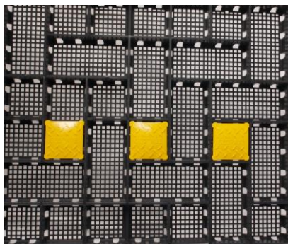
Figure 2. GEOPAVE SNAP Delineators installed in GEOPAVE Unit
